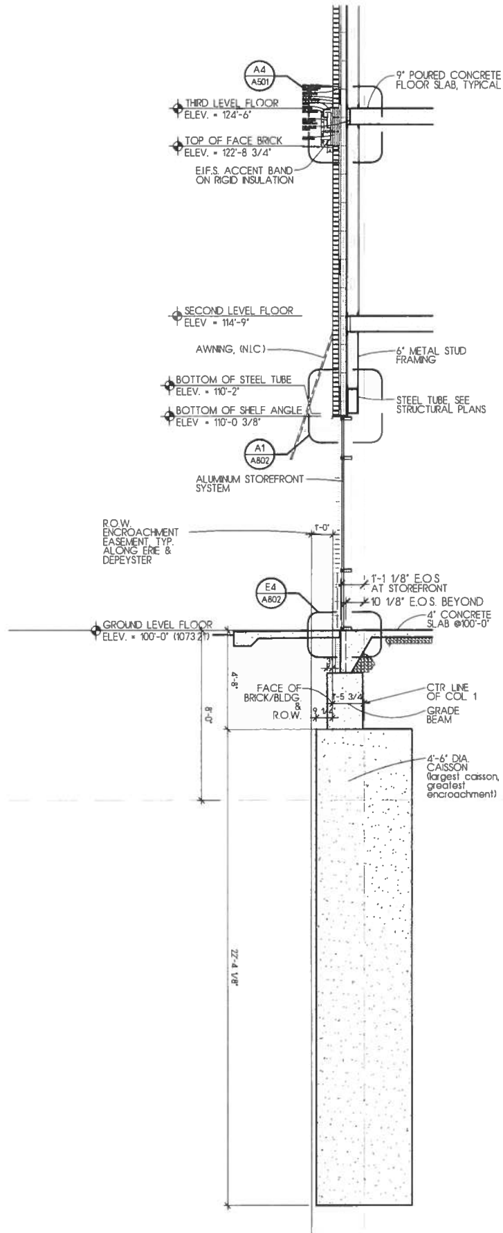
TYPICAL WALL SECTION @ ERIE STREET
